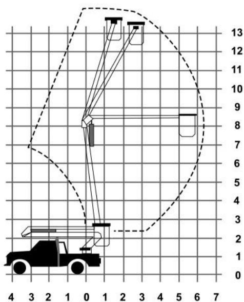
Diagrama de Alcances VAM 175/13 - 175/13 A
